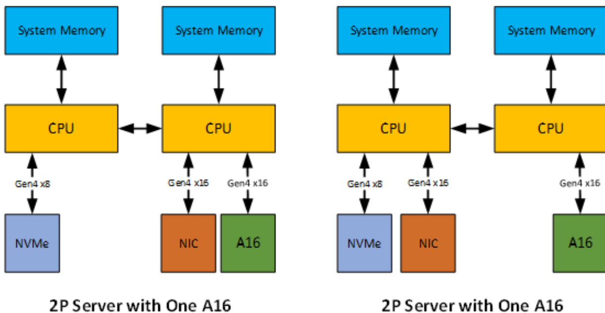
Figure 10. 2P Server with One NVIDIA A16 Card
