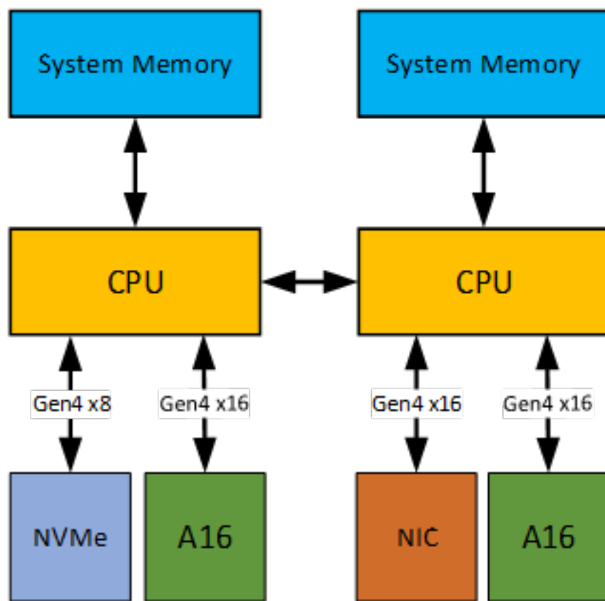
2P Server with Two A16s
