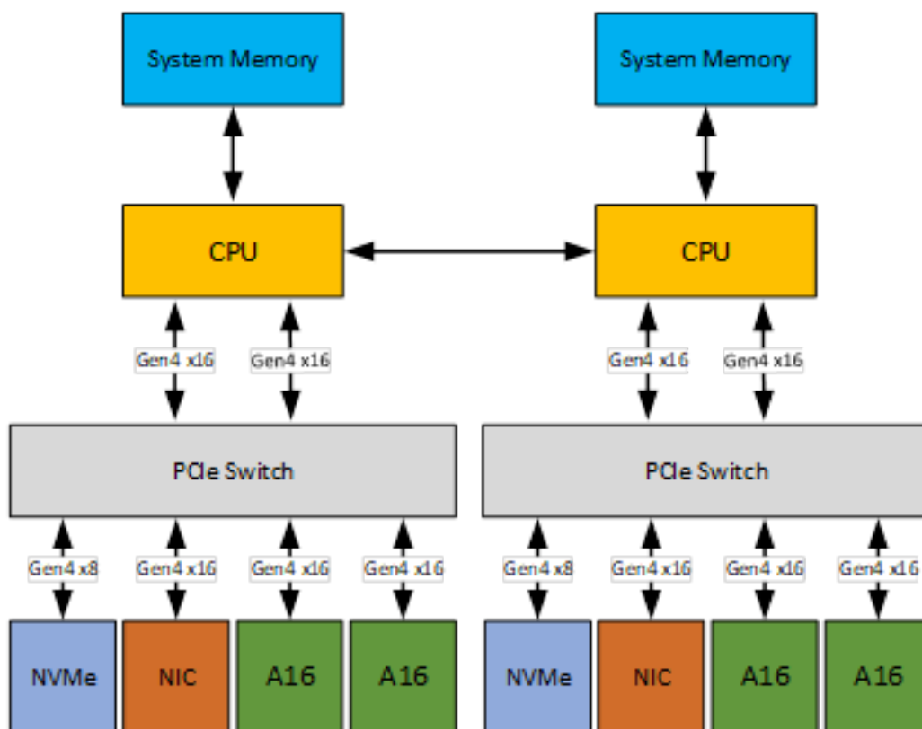
Figure 13. 2P Server with Four NVIDIA A16 Cards
