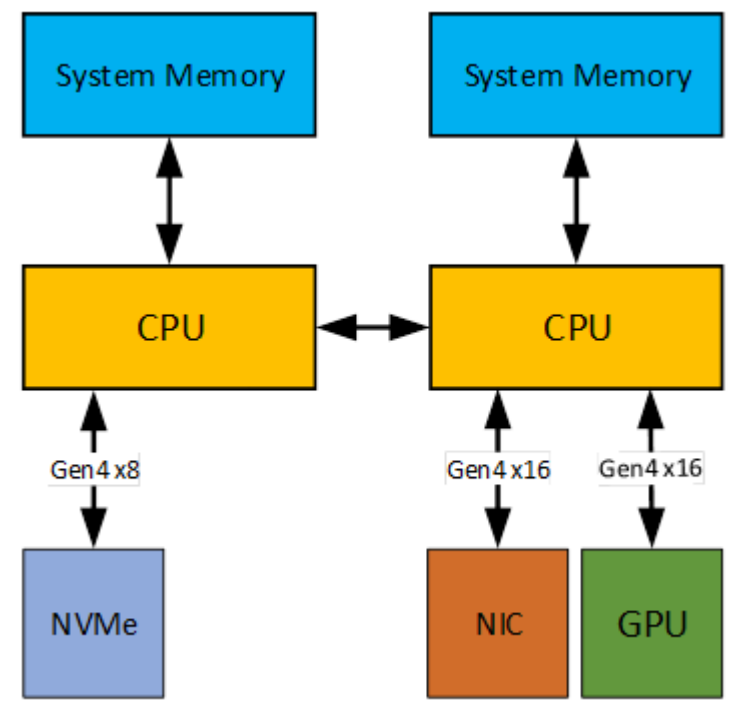
Figure 3. 2P Server with One GPU
