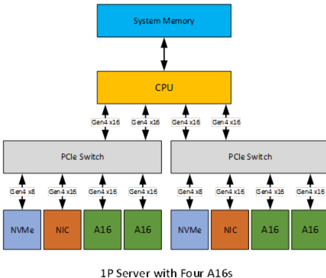
Figure 12. 1P Server with Four NVIDIA A16 Cards
