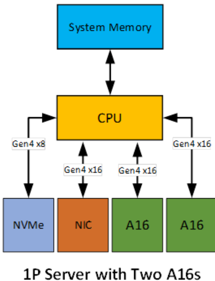
Figure 9. 1P Server with Two NVIDIA A16 Cards
