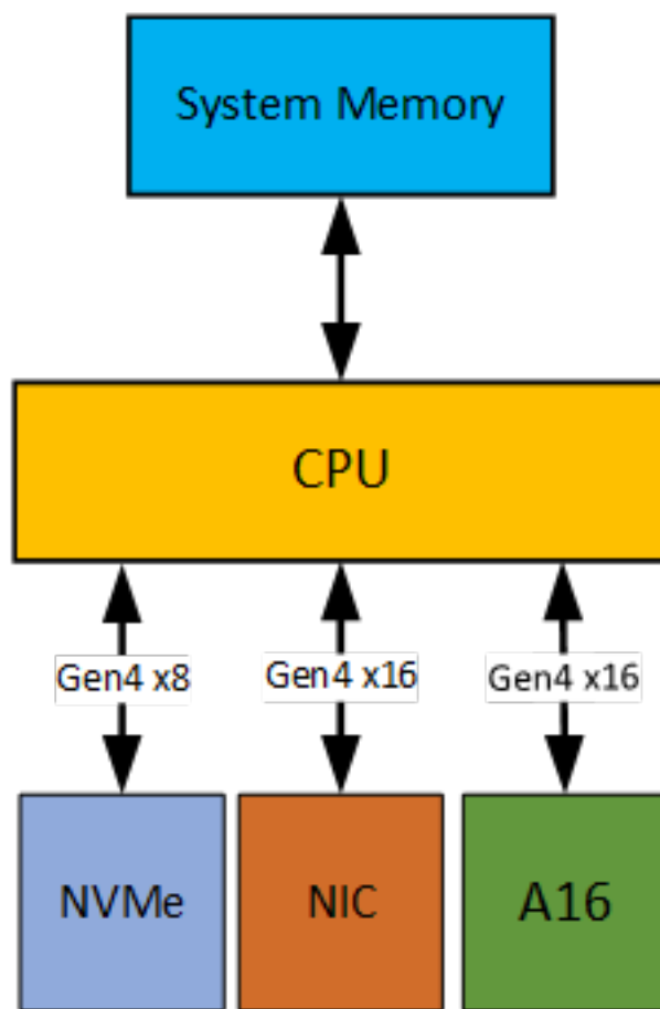
Figure 8. 1P Server with One NVIDIA A16 Card
