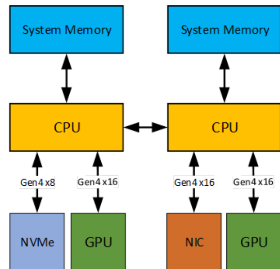
Figure 4. 2P Server with Two GPUs
