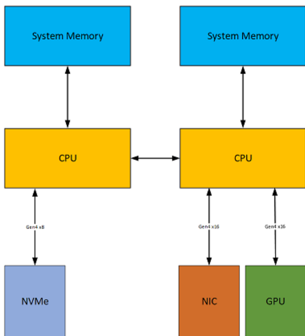
Figure 3. 2P Server with One GPU
